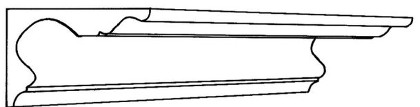
CP199 Projection 138mm(5 3/8") Depth 95mm(3 3/4")
