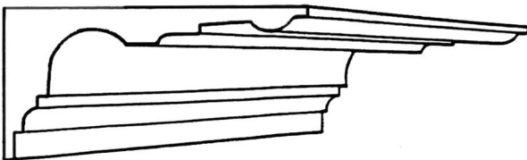
CP66 Projection 178mm(7") Depth 110mm(4 3/8")
