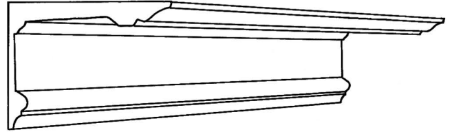
CP191 Projection 170mm(6 5/8") Depth 130mm(5 1/4")
