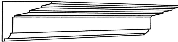
CP174 Projection 160mm(6 3 / 8 ") Depth 130mm(5 1 / 8 ")
