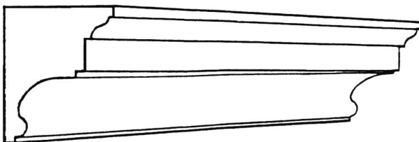
CP46 Projection 86 mm (3 3/8") Depth 108 mm (4 1/4")
