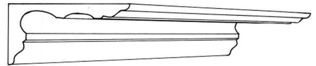
CP207 projection 206mm( 8\frac{1}{8} "") depth 105mm( 4\frac{1}{8} "")
