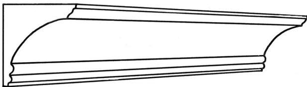
CP136 Projection 95mm(33/4") Depth 108mm(41/4")
