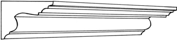
CP202 projection 100mm(4"") depth 75mm( 2\frac{7}{8} "")
