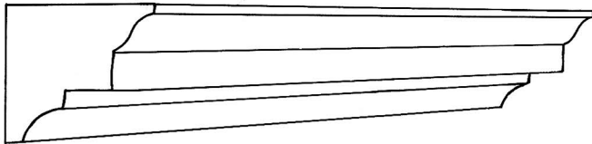
CP194 Projection 75mm(3") Depth 70mm(2 3/4")
