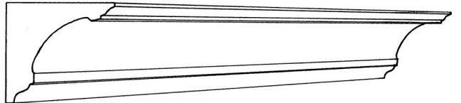
CP215 Projection 165mm(6 1 / 2 " ) Depth 155mm(6 1 / 8 " )
