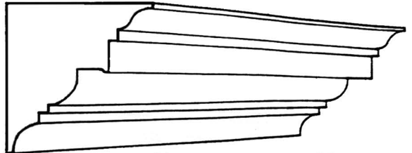
CP63 Projection 130mm(5 1/8") Depth 124mm(4 7/8")
