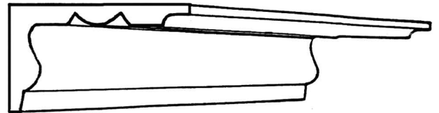
CP65 Projection 140mm(5 1/2") Depth 86mm(3 3/8")
