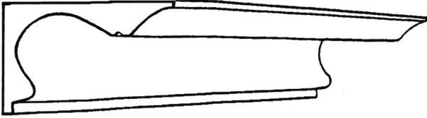
CP50 Projection 127mm(5") Depth 90mm(3 1/2")
