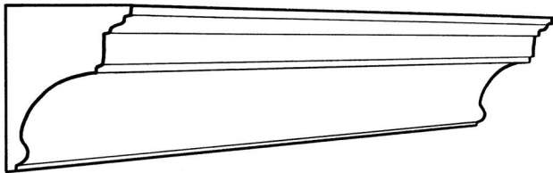
CP112 Projection 83mm(3 1 / 4 " Dpth 110mm(4 3 / 8 "
