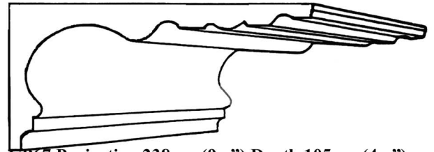
CP67 Projection 238mm(9 3/8") Depth 105mm(4 1/8") CP67a Projection 190mm(7 1/2") Depth 85mm(3 1/4") CP67b Projection 340mm(11 3/4") Depth 126mm(5")
