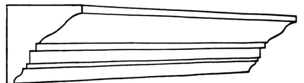
CP49 Projection 83 mm (3 1/4") Depth 89 mm (3 1/2")
