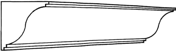
CP62 Projection 92mm(3 5/8") Depth 92mm(3 5/8") CP62a Projection 68mm(2 5/8") Depth 68mm(2 5/8") CP62b Projection 105mm(4 1/8") Depth 105mm(4 1/8")
