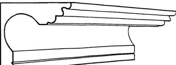
CP68 Projection 130mm(5 1/8") Depth 127mm(5")
