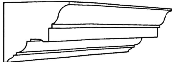
CP55 Projection 170mm(6 3/4") Depth 165mm(6 1/2")
