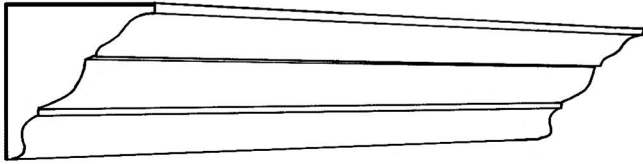
CP190 Projection 90mm(3 1/2") Depth 95mm(3 3/4")
