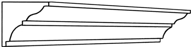
CP126 Projection 82mm(3 1 / 4 "") Depth 80mm(3 1 / 8 "")
