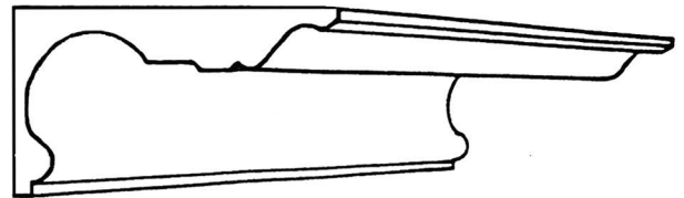
CP77 Projection 162mm(6 3 / 8 ") Depth 98mm(3 7 / 8 ")
