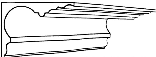
CP78 Projection 170mm(6 5 / 8 ") Depth 115mm(4 1 / 2 ") CP78a Projection 195mm(7 5 / 8 ") Depth 135mm(5 1 / 4 ") CP78b Projection 137mm(5 3 / 8 ") Depth 95mm(3 3 / 4 ")
