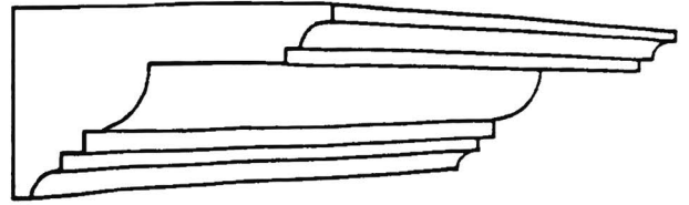
CP51 Projection 159mm(6 1/4") Depth 95mm(3 3/4")
