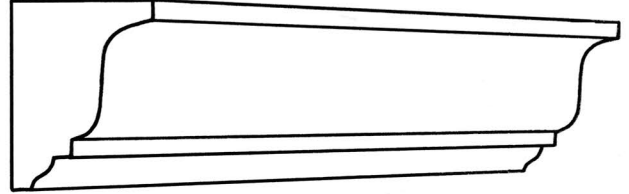
CP121 Projection 65mm(2 1 / 2 "") Depth 86mm(3 1 / 2 "")
