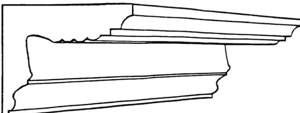
CP48 Projection 143 mm (5 5/8") Depth 117 mm (4 5/8")
