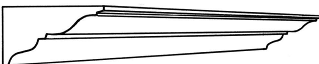
CP108 Projection 138mm(5 3 / 8 "") Depth 82mm(3 1 / 4 "")
