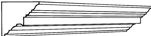
CP146 Projection 100mm(4") Depth 92mm(3 5 / 8 ")
