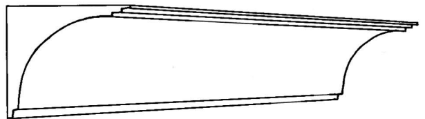
CP197 Projection 145mm(5 3/4") Depth 130mm(5 1/8")
