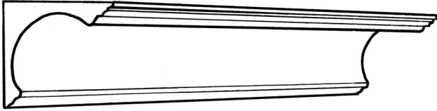
CP110 Projection 226mm(9") Depth 220mm(8 3 / 4 "
