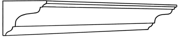
CP131 Projection 148mm(6") Depth 120mm(43/4") CP131a Projection 100mm(4") Depth 80mm(31/8")
