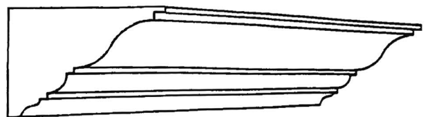
CP59 Projection 124mm(4 7/8") Depth 92mm(3 5/8")
